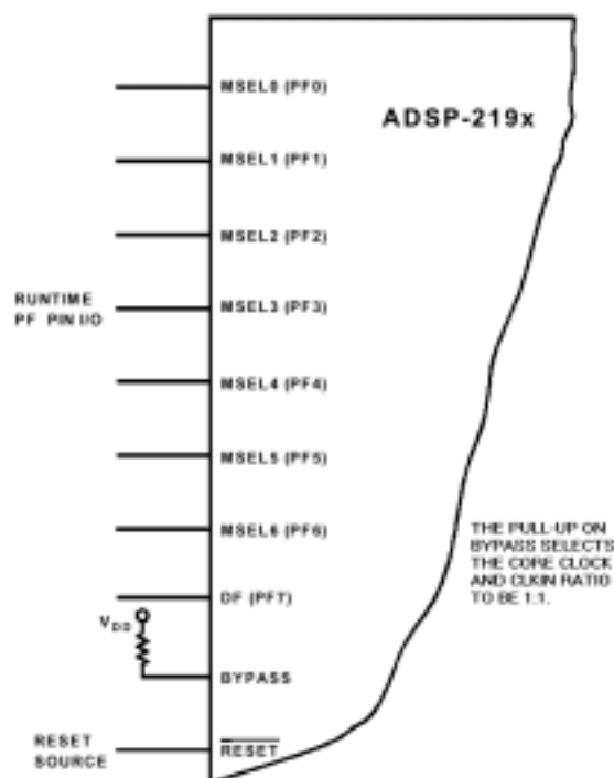
Figure 2. BYPASS pin termination.
